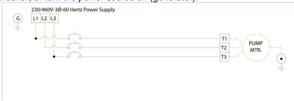
Typical 3 Phase Manual Control 1
