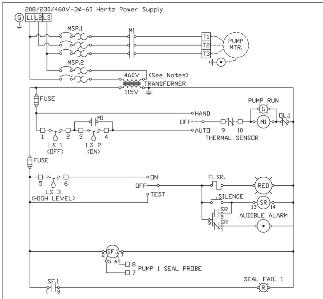
Typical 3 Phase Auto Control 1
